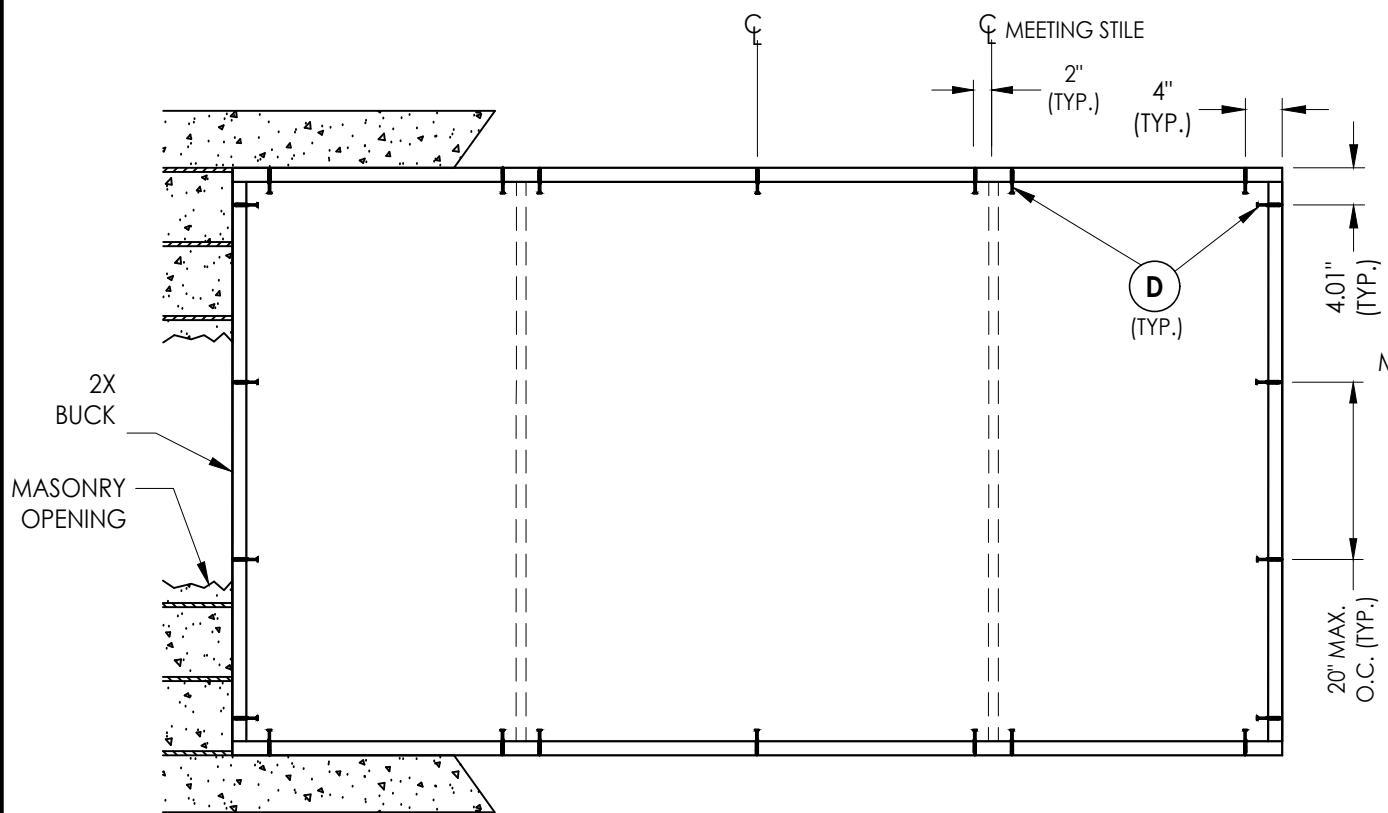
BUCK ANCHORING
