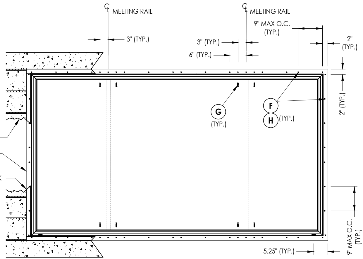
FRAME ANCHORING
